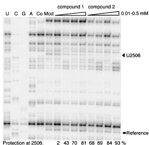
Figure 3. Gel analysis of protection of CMCT modification at nucleotide 2506. Lane U, C, G, A indicate the 23S RNA sequence in the analysed region. Co denotes a ribosomal RNA control lane. Mod. denotes RNA from CMCT modified ribosomes. The triangles are from ribosomes complexed with compounds at 0.01, 0.05, 0.2 and 0.5 mM, respectively, and treated with CMCT. The protections are normalised to the indicated reference band.
