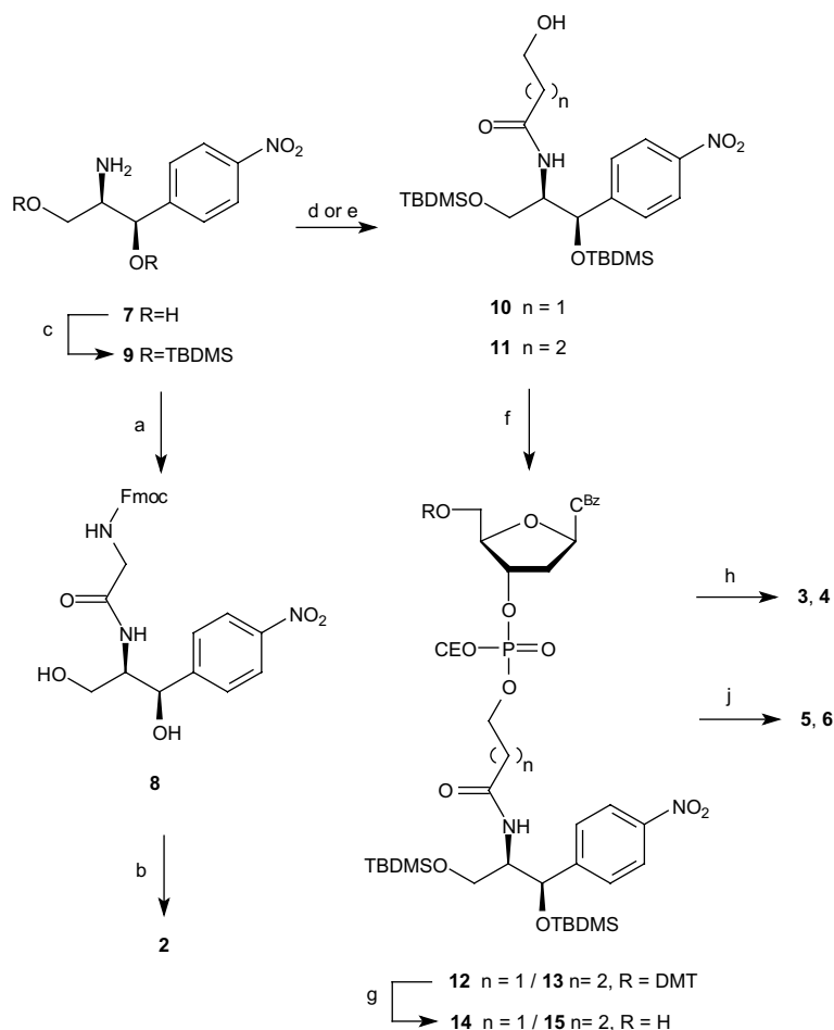
Scheme 1. Reagents and conditions: (a) Fmoc-Gly-OC 6 F 5 , CH 3 CN, 95%; (b) i, Et 3 N, DMF; ii, (1-pyrenyl)acetic acid, DCC, NHS, DMF, 39%; (c) TBDMS-OTf, 2,6-lutidine, CH 2 Cl 2 , 94%; (d) \beta -propiolactone, 2,6-lutidine, CH 2 Cl 2 , 10 24%; (e) \gamma -butyrolactone, 11 66%; (f) dC-CE/DMT phosphoramidite, 1 H -tetrazole, CH 3 CN then I 2 , aq pyridine, 12 48%, 13 34%; (g) TFA, CHCl 3 , Et 3 SiH, CH 2 Cl 2 , 14 45%, 15 54%; (h) i, TBAF, THF; ii, 32% aq NH 3 , HPLC, 3 38%, 4 58%; (j) i, dC-CE/DMT phosphoramidite, 1 H -tetrazole, CH 3 CN then I 2 , aq pyridine, 30%, 28%; ii, TFA, CHCl 3 , Et 3 SiH, CH 2 Cl 2 , 52%, 52%; iii, TBAF, THF; iv, 32% aq NH 3 , HPLC, 5 47%, 6 70%. C Bz = N -4-benzoylcytosine-1-yl, TBDMS = tert -butyldimethylsilyl, CE = 2-cyanoethyl, DMT = 4,4'-dimethoxytrityl.
