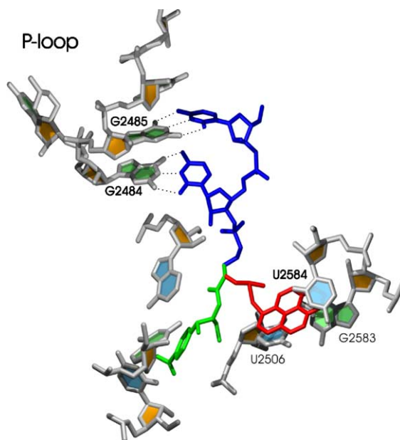
Figure 2. A combination of the two chloramphenicol conjugate types are shown with the chloramphenicol part in green, the pyrene (compound 2 ) in red and two cytidine residues (compound 6 ) in blue. Relevant 23S RNA nucleotides are shown as labelled ( E. coli numbering). Predicted hydrogen bonds to P-loop nucleotides are indicated.
