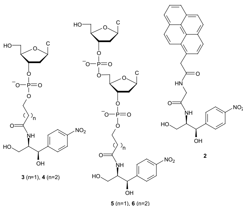
Figure 1. The designed pyrene and nucleotide chloramphenicol conjugates. C = cytosine-1-yl.
